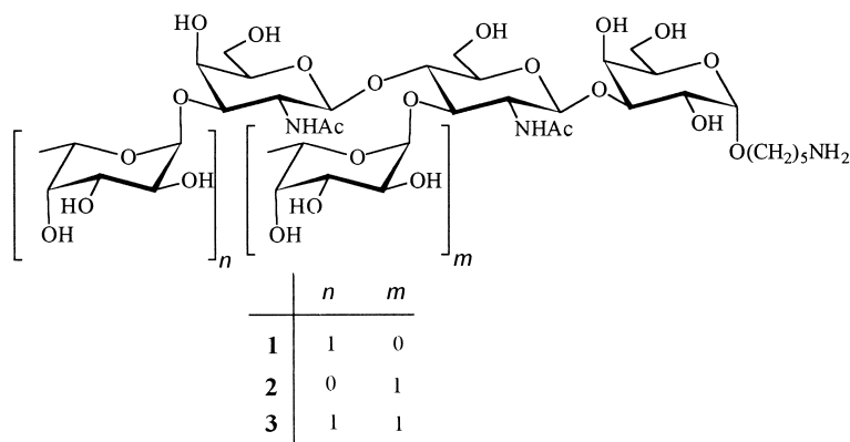
Figure 1. Synthesized oligosaccharide fragments of the glycocalyx glycan.
