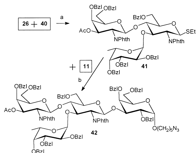
Scheme 7. a) AgOTf, 4 Å, DCM, sym -collidine, toluene, -30^{\circ}\text{C} ; b) MeOTf, 4 Å, \text{Et}_2\text{O} , 0^{\circ}\text{C} .
