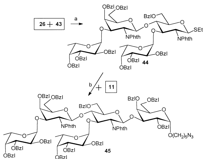
Scheme 8. a) AgOTf, 4 Å, DCM, sym -collidine, toluene, -30^{\circ}\text{C} ; b) MeOTf, 4 Å, \text{Et}_2\text{O} , 0^{\circ}\text{C} .
